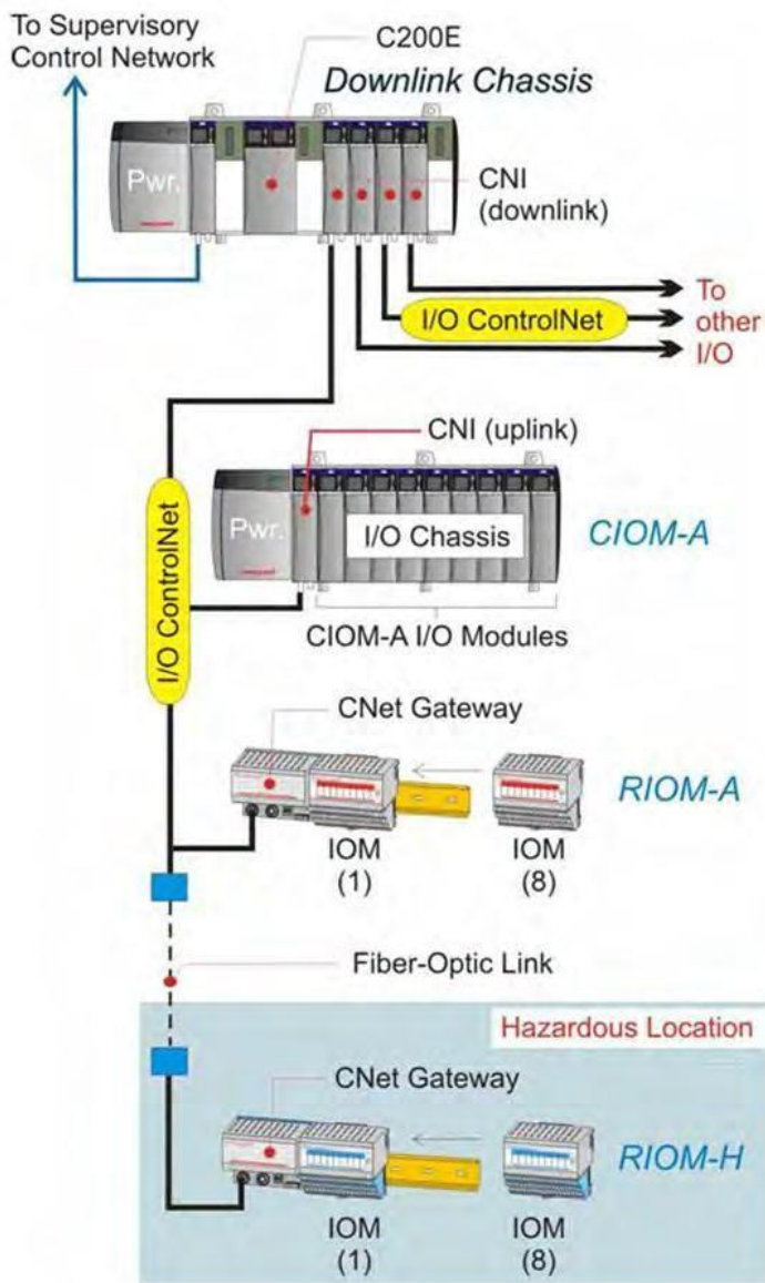
Figure 3-1 I/O Control Network Overview
