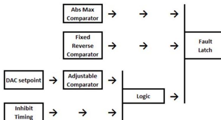
Figure 5. Block Diagram multiple comparators on a CT analog channel, including remotely programmable comparator threshold and inhibit timing.
