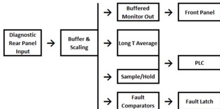
Figure 1. Block Diagram of one analog channel.
