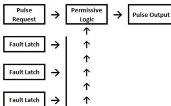
Figure 2. Block Diagram of fault logic permitting pulse pass-thru.
