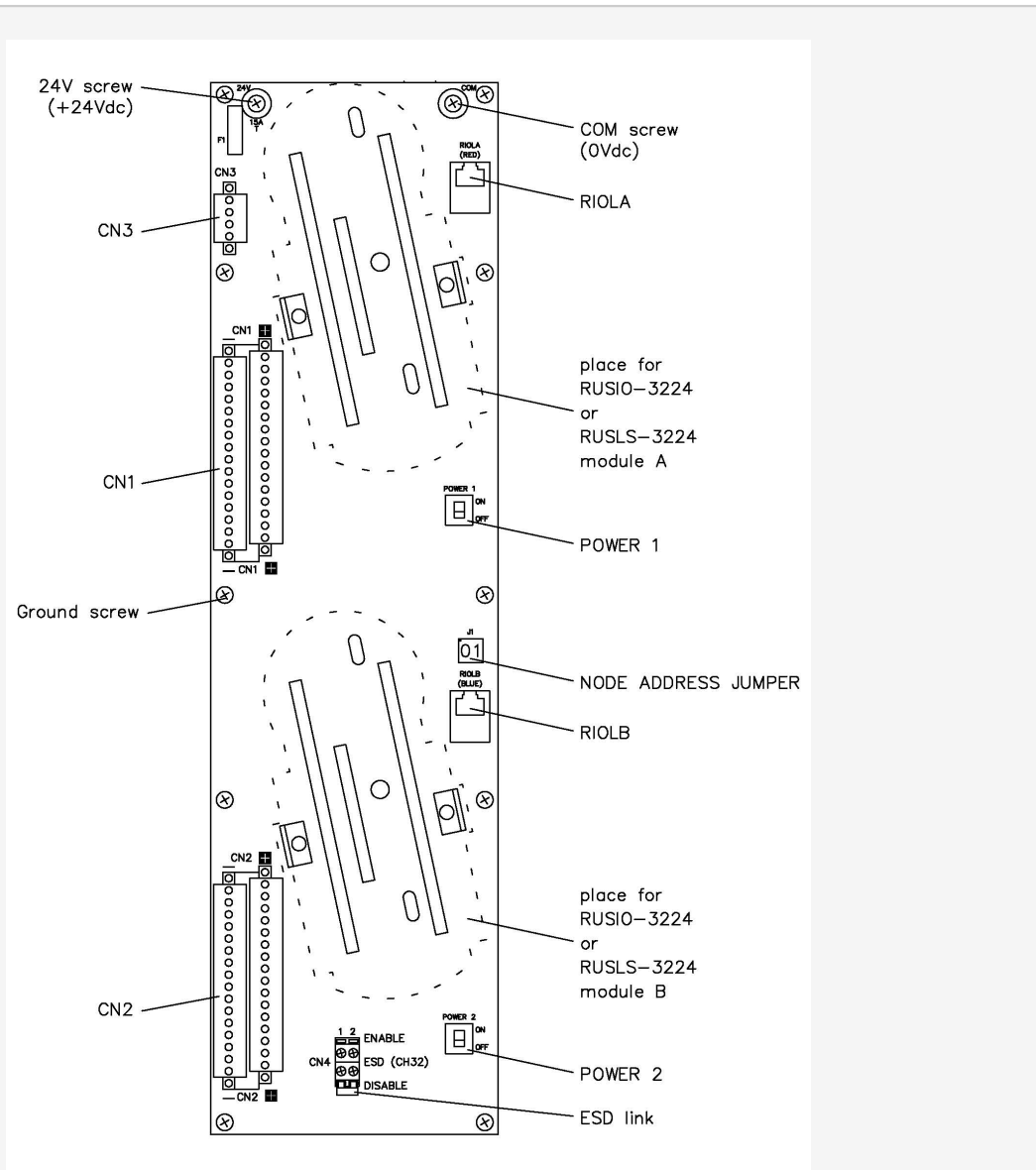
Figure 15-17: Mechanical layout
