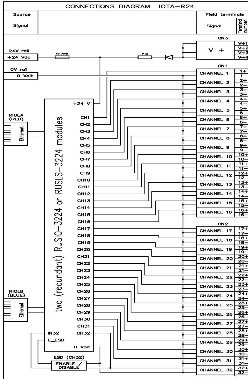
Figure 15-25: Connection diagram
