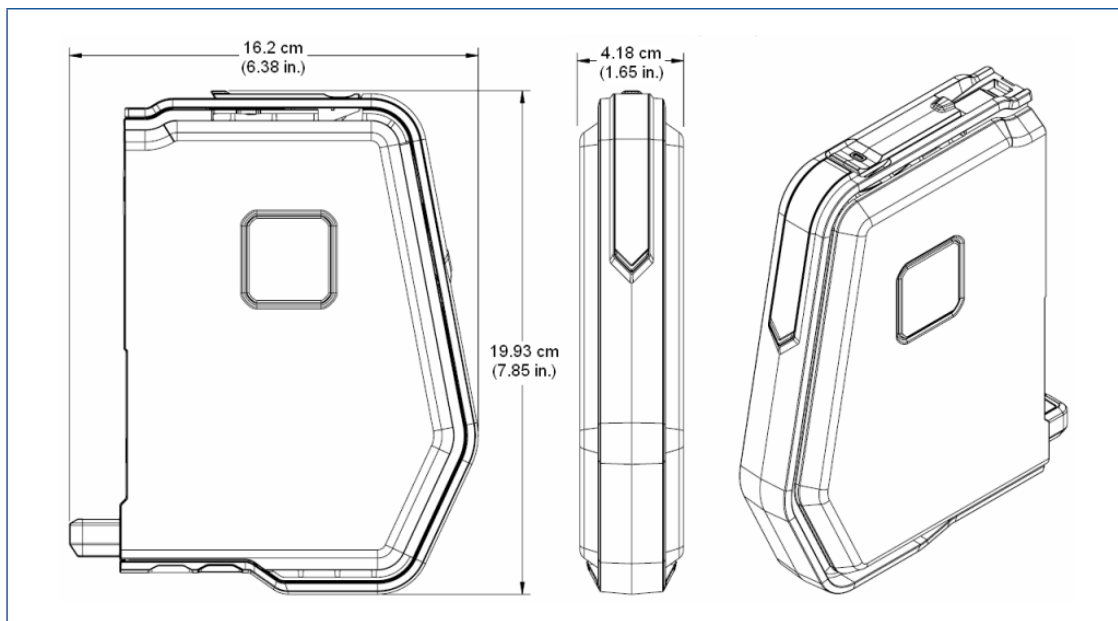
DeltaV SX Controller hardware dimensions.
