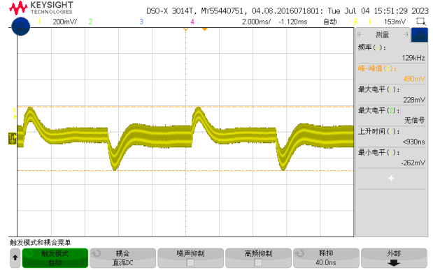
Figure 6, 50% - 75% load dynamic
