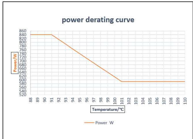
Figure 4, Power-Temperature
