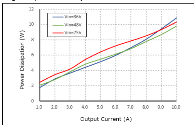
Figure 2, Power dissipation
