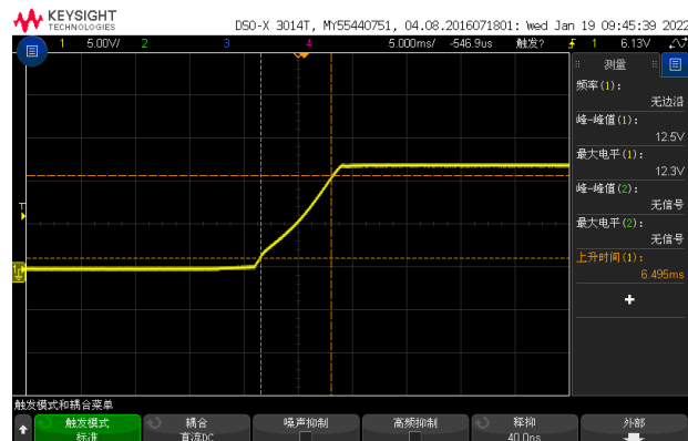
Figure 5, Output voltage established (Iout = 10A)
