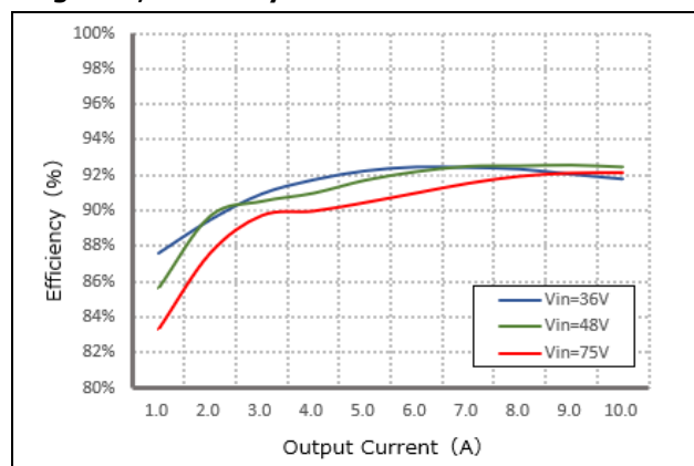
Figure 1, Efficiency
