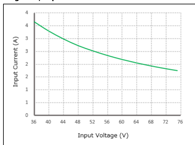
Figure 3, Input V-I
