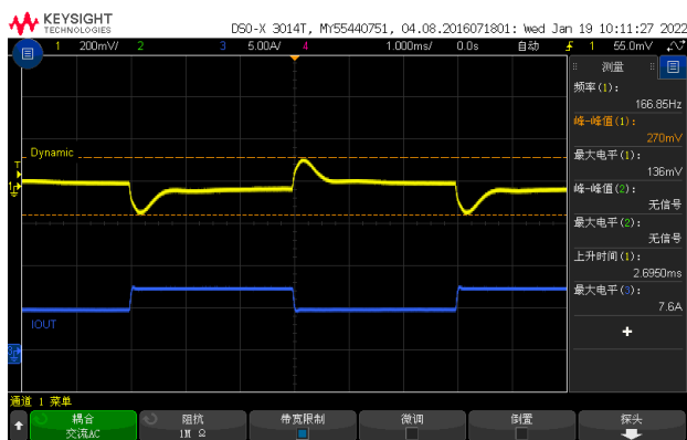
Figure 4, 50% - 75% load dynamic
