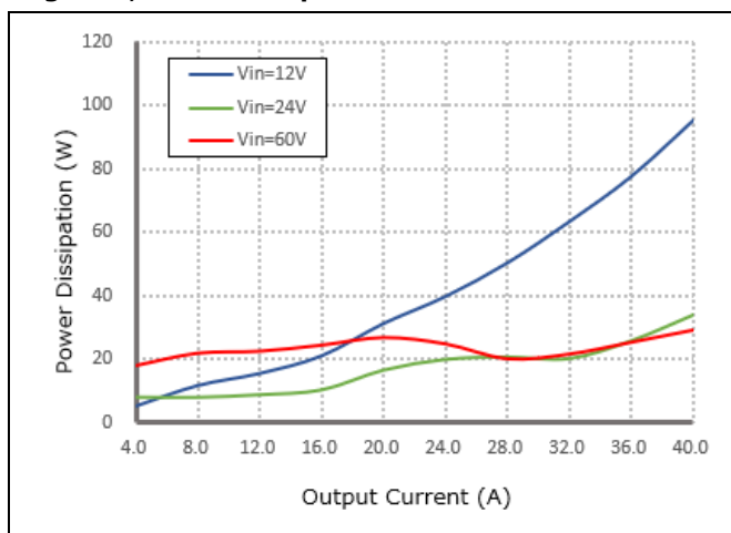
Figure 2, Power dissipation
