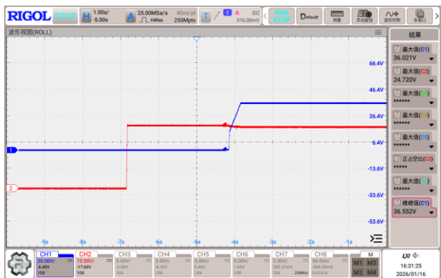
Figure 7, Output voltage established (Iout = 40A)
