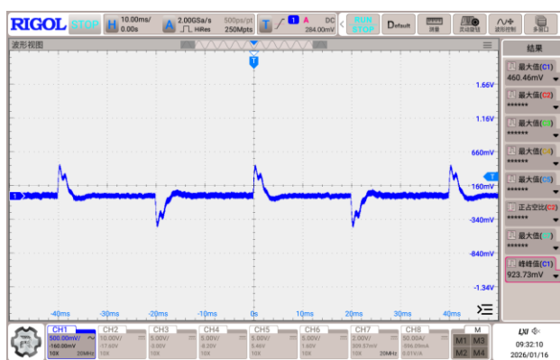
Figure 6, 50% - 75% load dynamic
