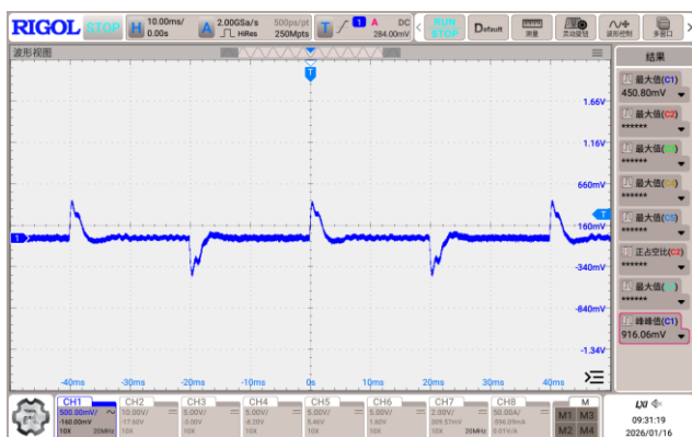
Figure 5, 25% - 50% load dynamic
