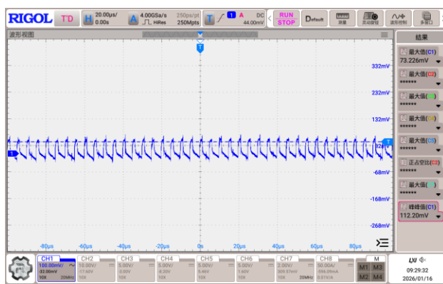
Figure 8, Output ripple & noise (Iout = 40A)
