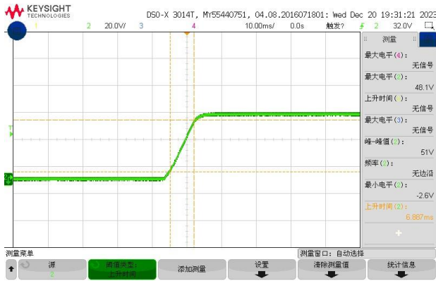
Figure 6, Output voltage established (Iout = 4A)
