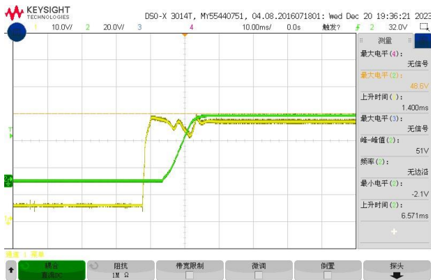
Figure 8, Boot delay time (Iout = 4A)
