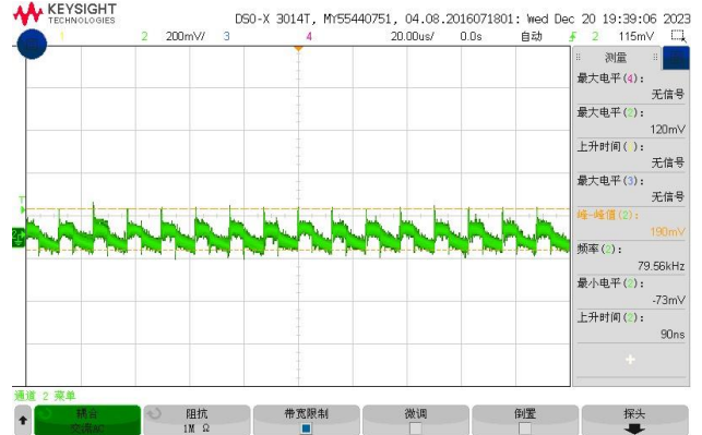
Figure 7, Output ripple & noise (Iout = 4A)
