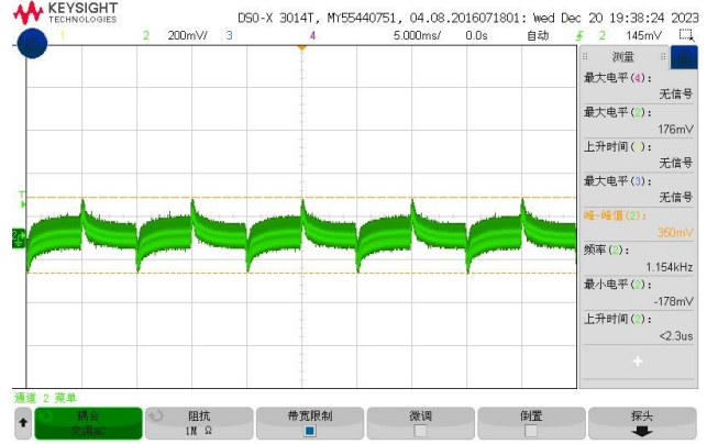
Figure 5, 50% - 75% load dynamic
