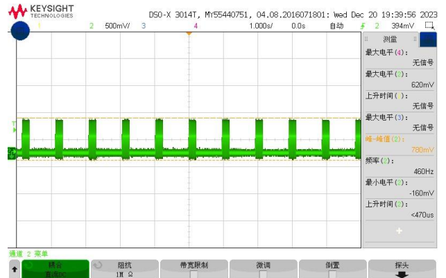
Figure 9, Short circuit & Out voltage (Iout = 4A)
