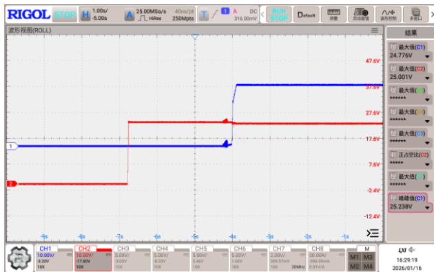
Figure 7, Output voltage established (Iout = 60A)
