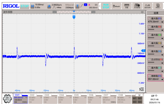
Figure 6, 50% - 75% load dynamic
