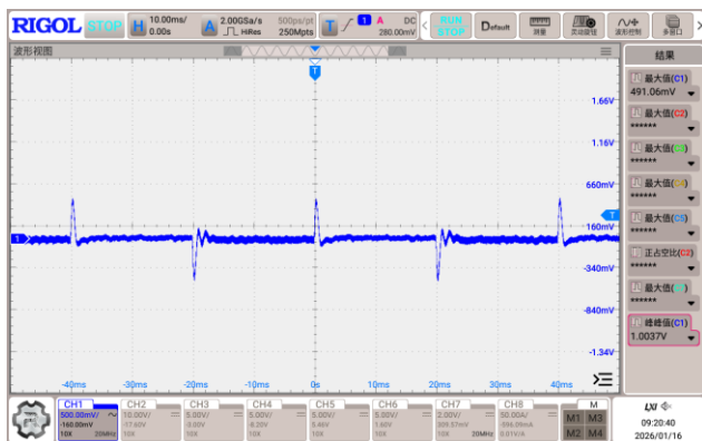
Figure 5, 25% - 50% load dynamic
