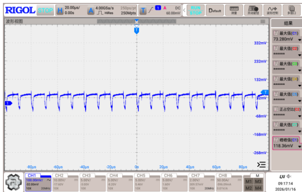
Figure 8, Output ripple & noise (Iout = 60A)
