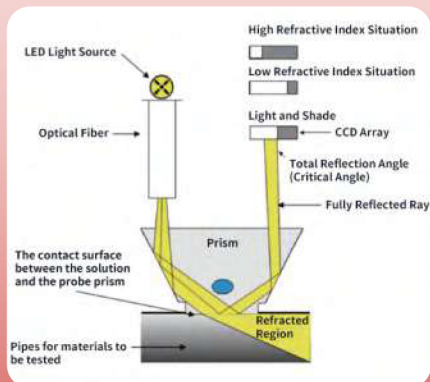
Measuring principle
