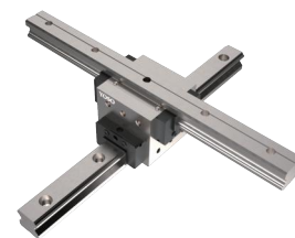
Cross configuration guide rail YS-CSR
