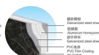
彩鋼板壁板結構 Colored Steel Wall Panel Structure
