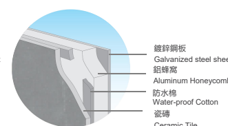
瓷磚壁板結構 Ceramic Tile Wall Panel Structure
