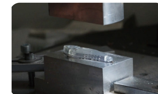
ULTRASONIC WELDING
