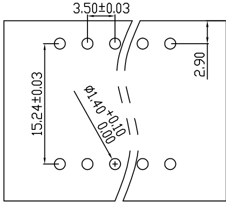
PCB LAYOUT
