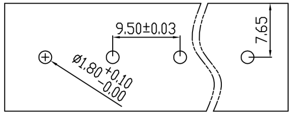
PCB LAYOUT
