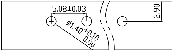
PCB LAYOUT
