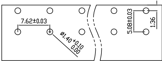
PCB LAYOUT
