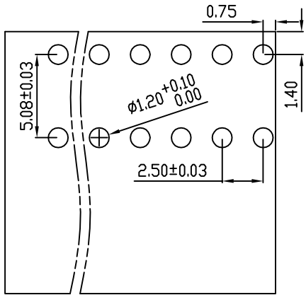
PCB Layout
