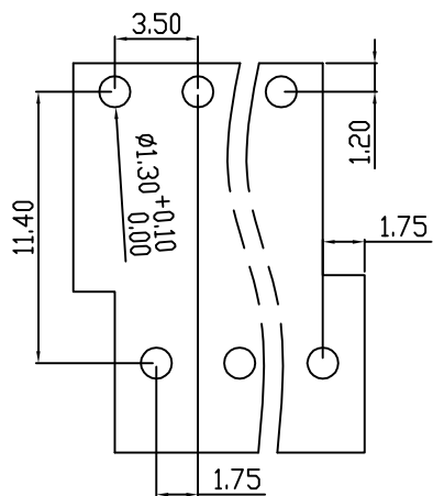
PCB Layout
