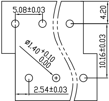
PCB LAYOUT
