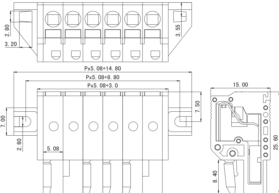
KFM508CP-5.08
