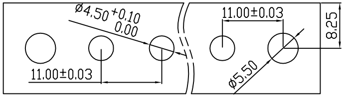
PCB LAYOUT
