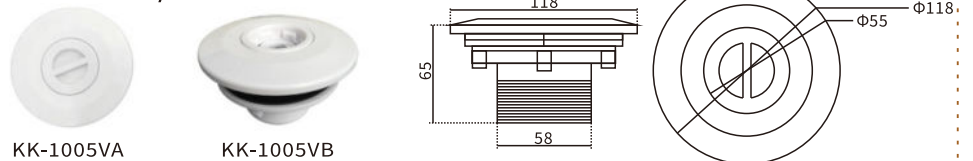
KK-1005VA/P
