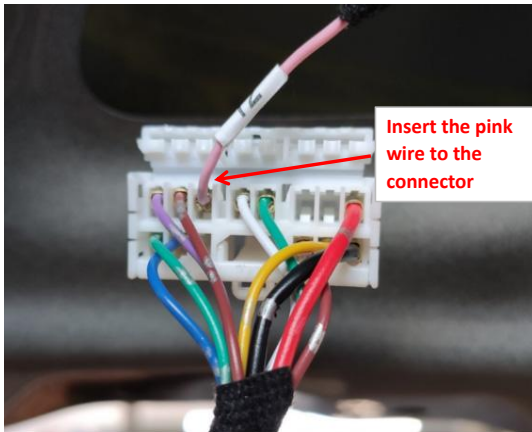
16. Insert the pink wire (No.12) into the indicated slot of the connector.
