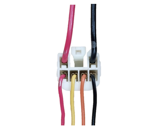
11. Insert the strut wiring harness terminals into the connector according to the diagram.
