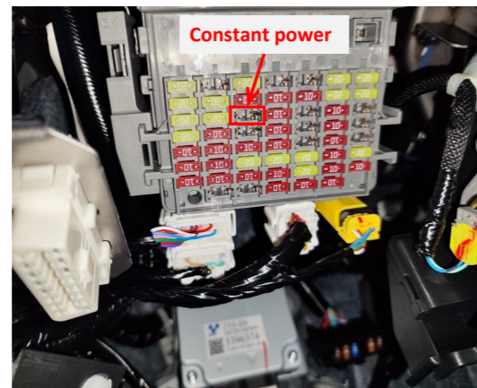
23. The fuse box is located at the driver's position and the fuse slot for power supply is indicated above.
