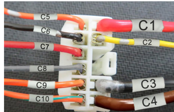
28. Insert the power harness terminals into the connector as indicated in the diagram.
