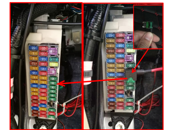
27. Move the indicated fuse (sixth in the rightmost column), to the fuse tap and then plug the fuse tap into the fuse box.
