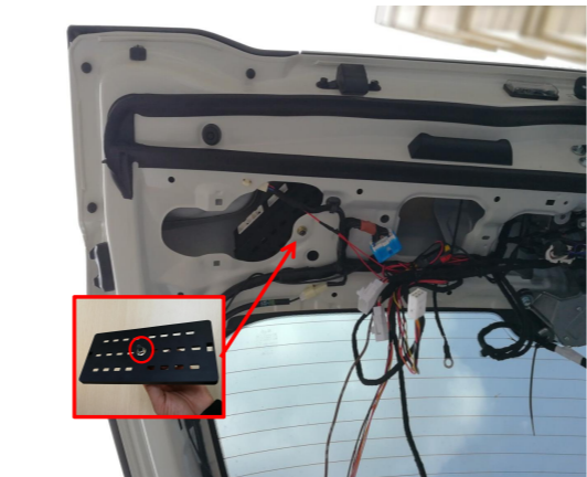
29. Screw a nut on the ECU bracket first and then fix it to the indicated hole.
