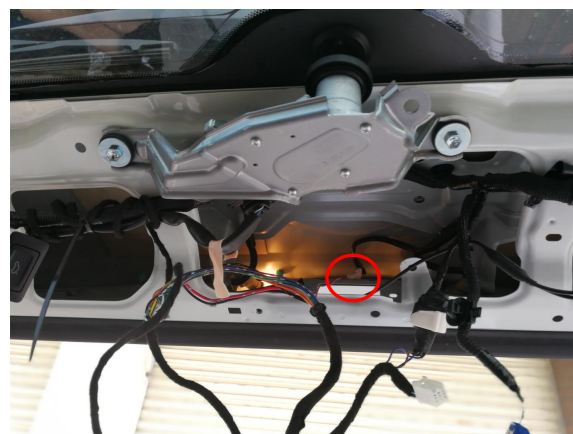
7. Connect the plugs of the lock signal harness to the original tailgate switch
