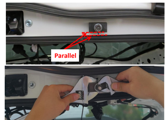
32. Install the hole opener (make sure its edge is parallel to the lower edge of the tailgate) and open the hole (one wrench holds the hole opener and the other wrench turns the nut).
