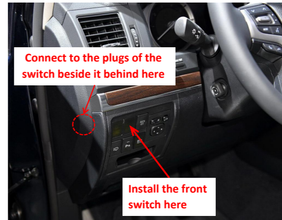
25. Remove the blank button from the switch panel and install the added front switch.
