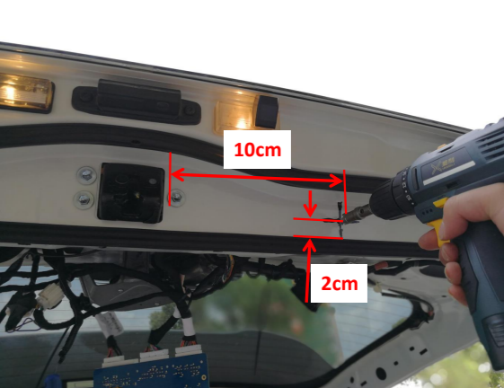
31. Drill a hole at the right side of the tailgate using a \phi 14mm drill bit.
