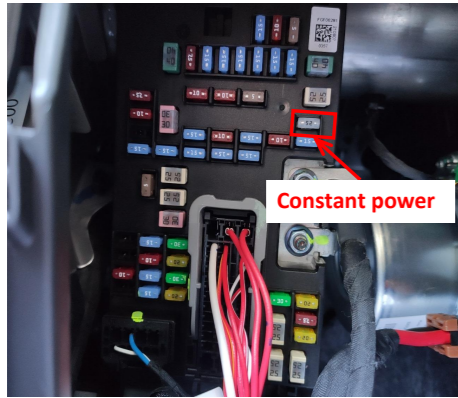
22. The fuse box is located behind the storage box at the driver's position and the slot for power supply is indicated above.
