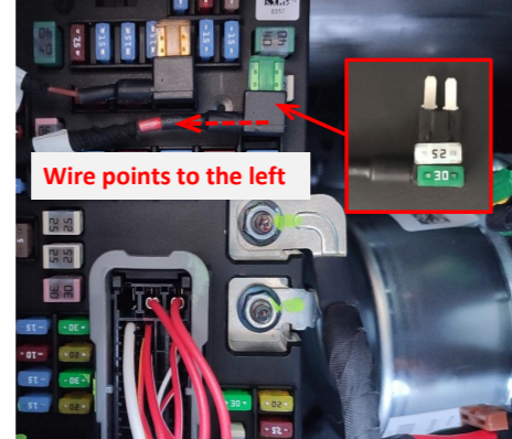
23. Move the fuse from the fuse box to the fuse tap and then plug the fuse tap into the fuse box. Pay attention to the direction.
