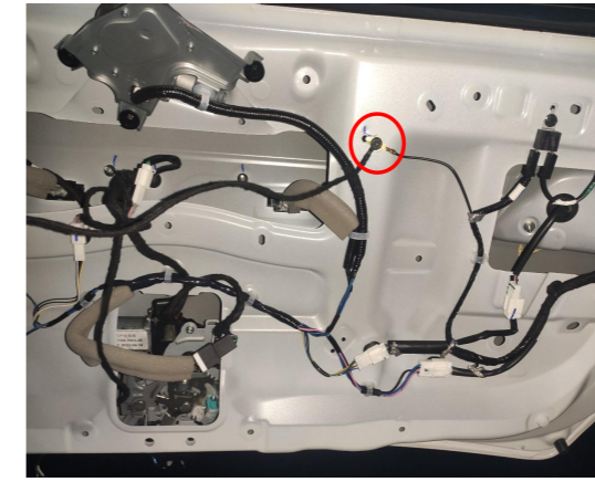
20. Ground at the indicated position on the tailgate with the ground wire connector.
