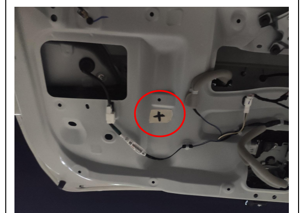
26. Drill a mounting hole at the indicated position with a \phi 6mm drill bit for the ECU bracket.
