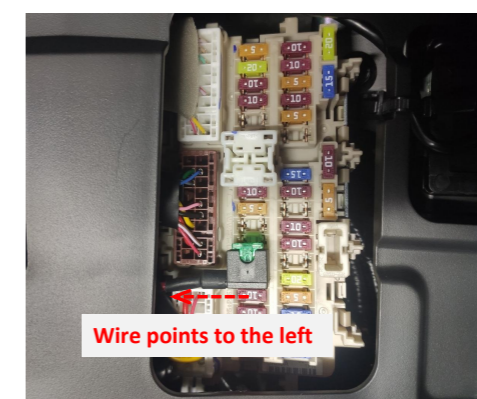
25. Move the original fuse from the fuse box to the fuse tap and then plug the fuse tap into the fuse box. Pay attention to the direction.
