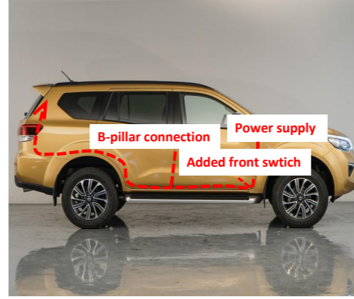
19. Route the power harness.
