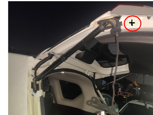
15. Drill a hole at the indicated position with a \phi 21\text{mm} drill bit to allow the strut wiring harness to pass through. Both the left and right sides are the same.
