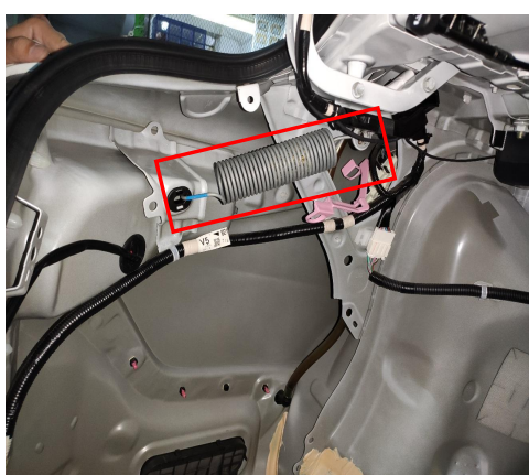
8. Remove the left and right springs from the trunk.
