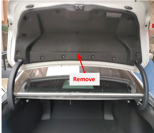
3. Remove the tailgate trim panel.
