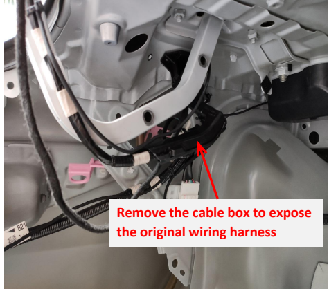
6. Remove the cable box from the left hinge to prevent interference.
