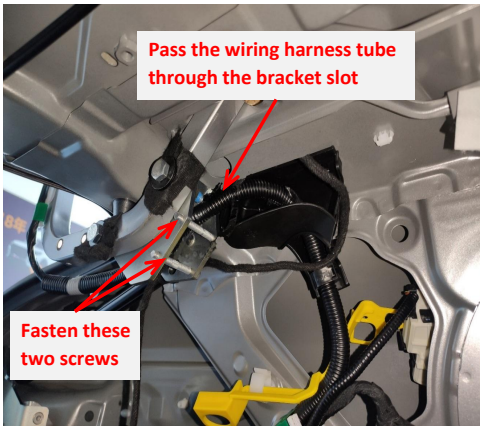
14. Pass the wiring harness tube through the bracket slot and fasten the two screws tightly.
