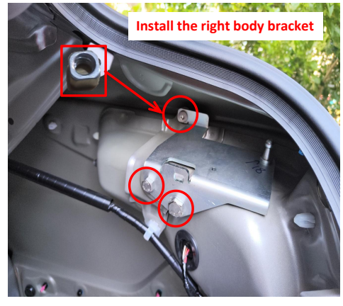
11. Install the right body bracket.
