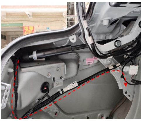
19. Route the left strut wiring harness along with orignal wires.
