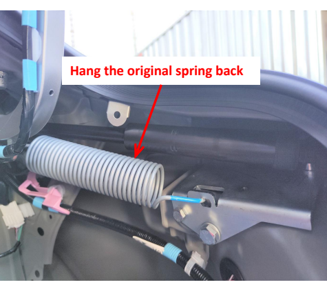
18. Hang the left and right springs back.(wrap the two end of the springs with velvet fabric to prevent abnormal soound during operation)
