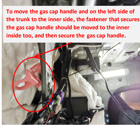
5. Move the gas cap handle on the left side of the trunk to the inner side to prevent interference.
