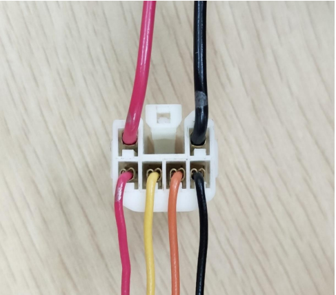
11. Insert the strut wiring harness terminals into the wiring harness connector.
