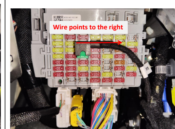
26. Plug the fuse tap into the fuse box and pay attention to the direction of wire.
