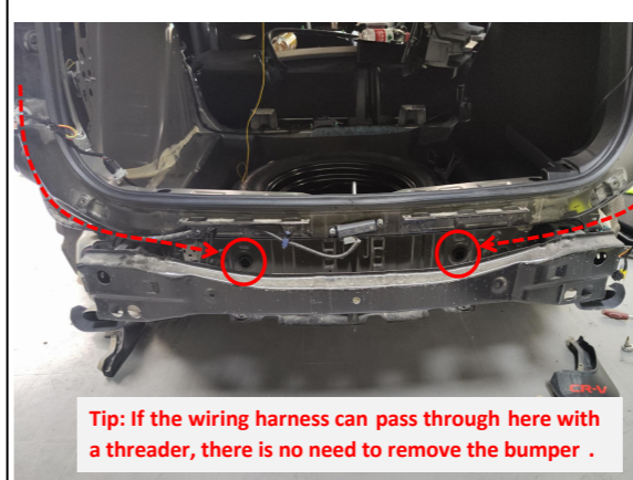
10. Remove the plugs from the holes and thread the strut wiring harnesses through the holes into the car body.
