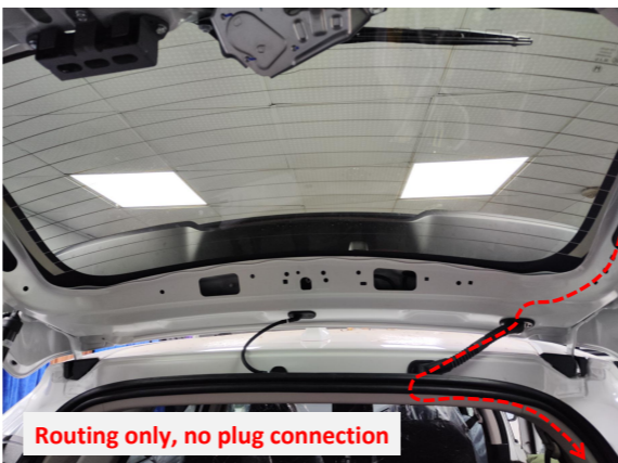
14. Route the lock signal harness to the right side of the trunk.
