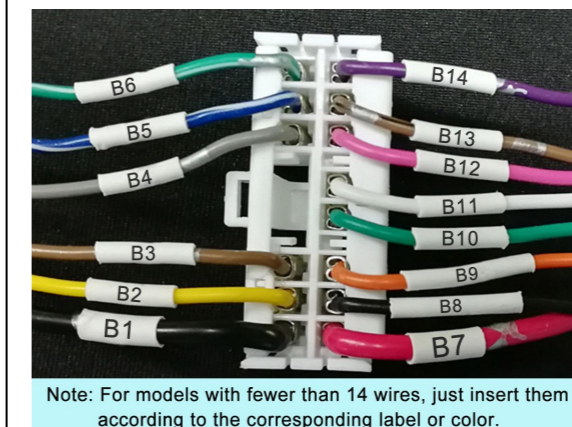
15. Insert the lock signal harness terminals into the wiring harness connector.
