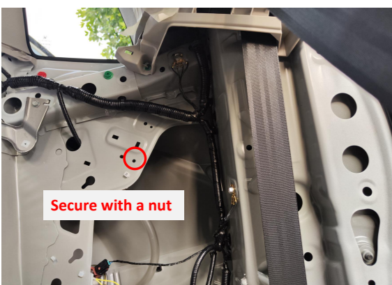
27. Secure the ECU at the right side of the trunk.
