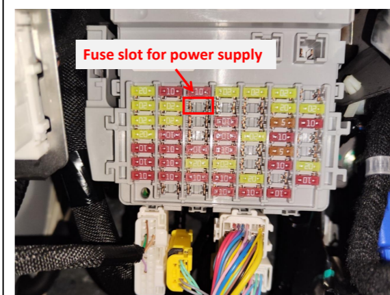
25. Connect to the fuse box for power supply.
