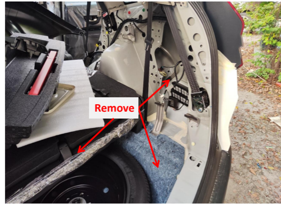
3. Take out the trunk floor mat and remove the trim panel on the right side of the trunk.
