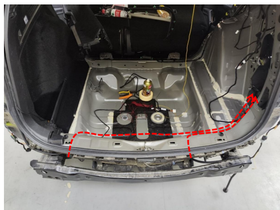
12. Route the strut wiring harnesses to the right side of the trunk.
