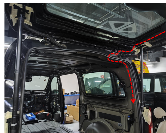
14. Route the lock signal harness to the right side of the trunk as indicated.
