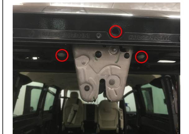
16. Remove the original latch.
