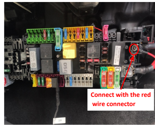
24. Connect to the indicated position with red wire connector for constant power (add a provided nut).
