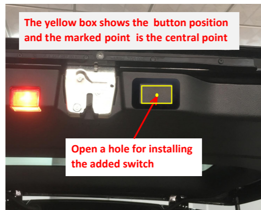
28. Stick the hole template to the indicated position and open a hole for the added tailgate switch.
