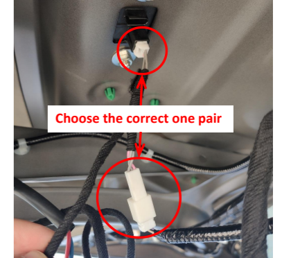
6. Connect the plugs of the lock signal harness with the plugs of tailgate handle switch (Due to configuration differences, two pairs of plugs have been reserved. Choose the correct one pair for connection).
