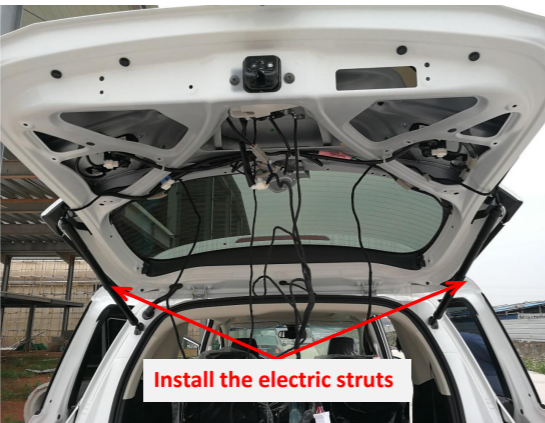
13. Install the electric struts, L on the left and R on the right (the first letter of the strut number).
