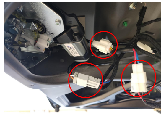
7. Connect the plugs of the lock signal harness with the plugs of the power latch.
