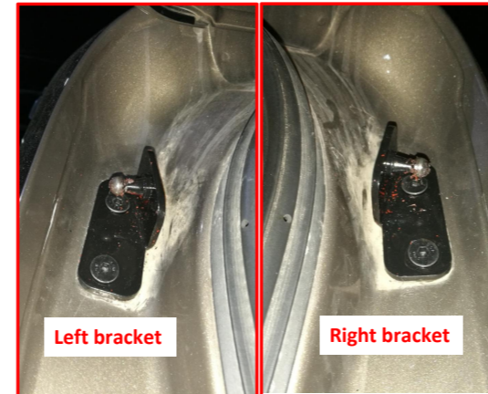
9. Replace the left and right body brackets.
