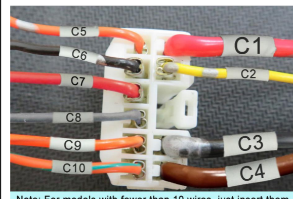
13. Insert the power harness terminals into the wiring harness connector. Note: For models with fewer than 10 wires, just insert them according to the corresponding label or color.
