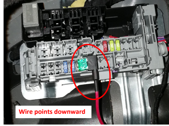
18. Plug the fuse tap into the fuse box and pay attention to the direction. Wire points downward
