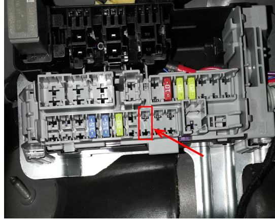
17. The slot for power supply (eighth in the second row).
