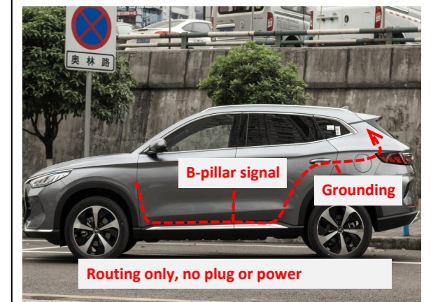
16. Route the power harness as indicated (routing only, no plug or power connection).
