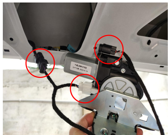
12. Connect the lock signal harness to the plugs of the power latch as shown above.
