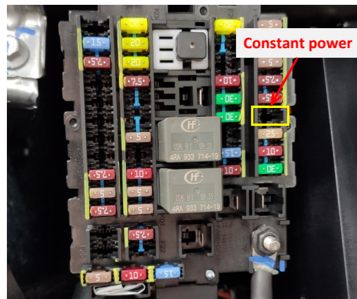
22. The fuse box is located at the driver's position and the fuse slot for power supply is indicated above.
