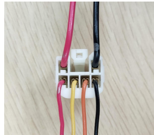
9. Insert the strut wiring harness terminals into the wiring harness connector as shown above.
