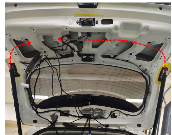
12. Thread the strut wiring harnesses into the tailgate.
