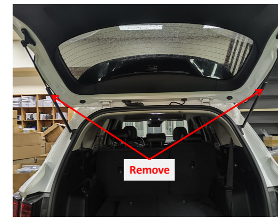
5. Remove the original gas struts.
