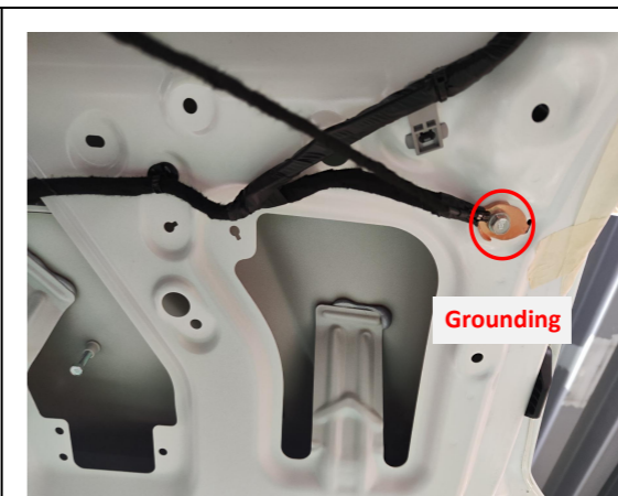
20. Ground at the indicated position of the tailgate.
