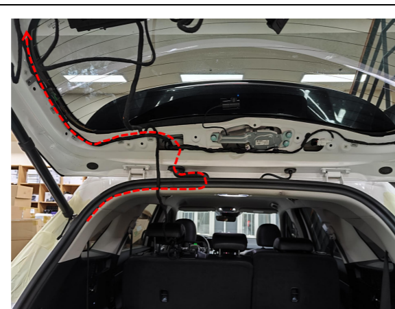
18. Thread the power harness to the tailgate.
