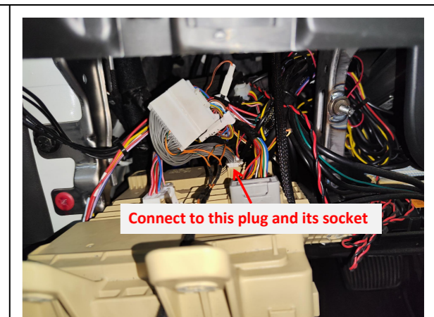
21. Connect to the CAN signal plug and its socket behind the fuse box.
