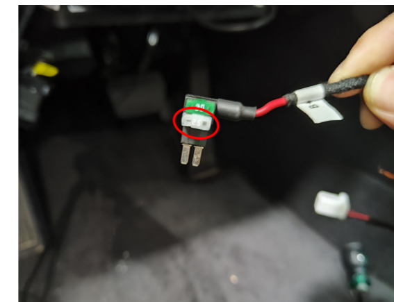
23. Move the fuse from the fuse box to the fuse tap.
