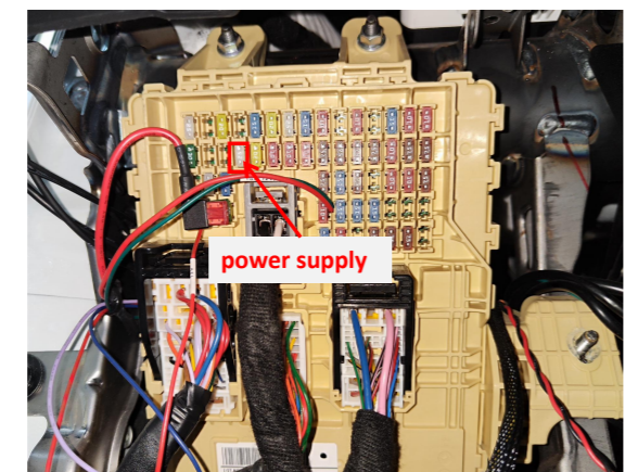
22. The fuse box is located at the driver's area and the fuse slot for power supply is indicated above.
