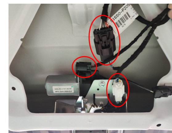
15. Connect the plugs of the lock signal harness to the plugs of the power latch and original latch.
