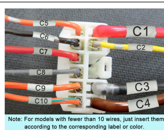
19. Insert the power harness terminals into the connector according to the diagram.
