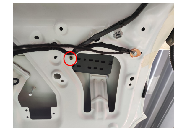
25. Secure the ECU at the indicated position.
