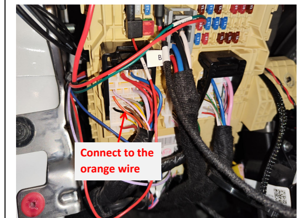
21-1. If you choose not to connect the CAN plugs, connect the orange wire of power harness to the indicated orange
