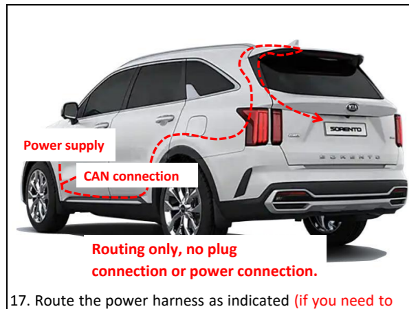
17. Route the power harness as indicated (if you need to install the added front switch, route the switch wiring harness in the same way).
