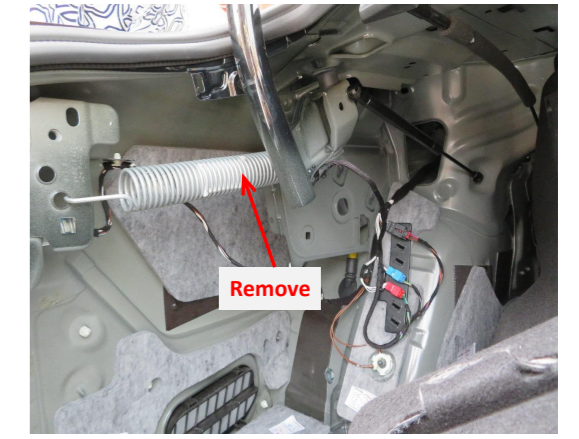
6. Remove the springs on both sides of the trunk.
