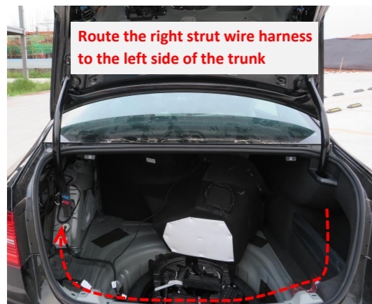
12. Route the right strut wiring harness to the left side of the trunk.
