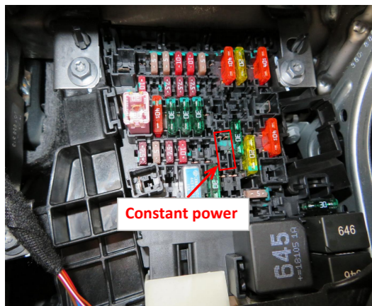
22. The fuse box is located beside the pedals and the slot for power supply is indicated above.
