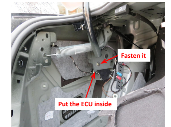
24. Secure the ECU at the indicated location with a nut.
