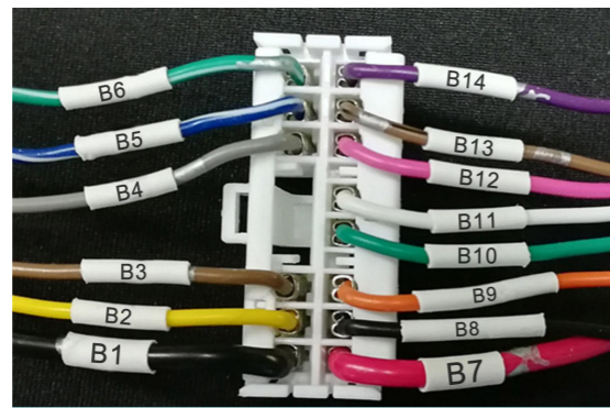
18. Insert the lock signal harness terminals into the connector as shown above.
