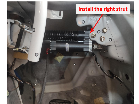
11. Install the right electric strut.
