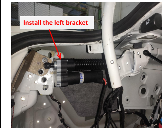
10. Install the left electric strut.
