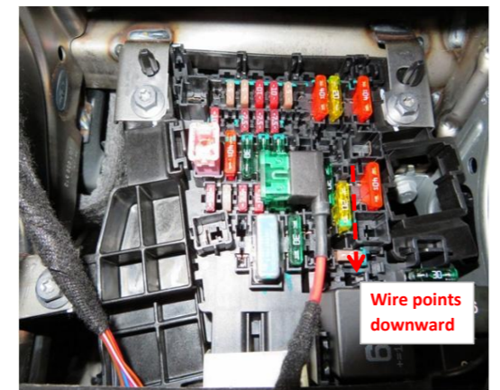
23. Plug the fuse tap into the fuse box. Pay attention to the direction of wire.
