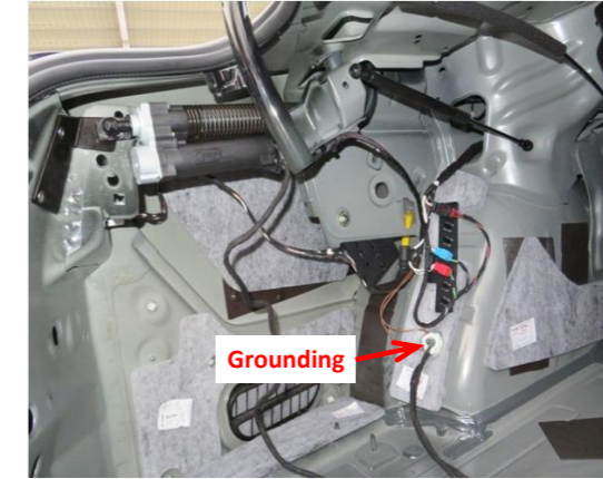
20. Ground at the indicated location on the left side of the trunk.
