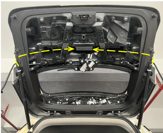
12. Thread the left and right strut wiring harness into the tailgate as indicated and plug the holes with rubber plugs.
