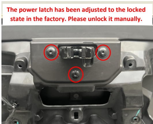
15. Install the power latch.
