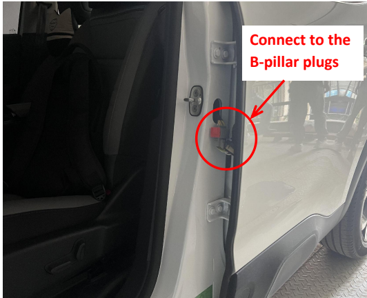
21. Connect to the B-pillar plugs at rear left B-pillar.
