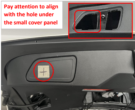
31. Stick the hole template to the indicated position and open a hole for the added tailgate switch.
