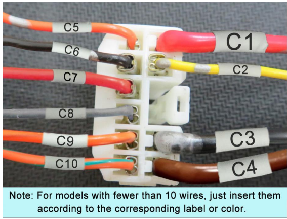
20. Insert the power harness terminals into the connector according to the diagram.
