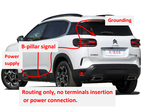
18. Route the power harness as indicated.
