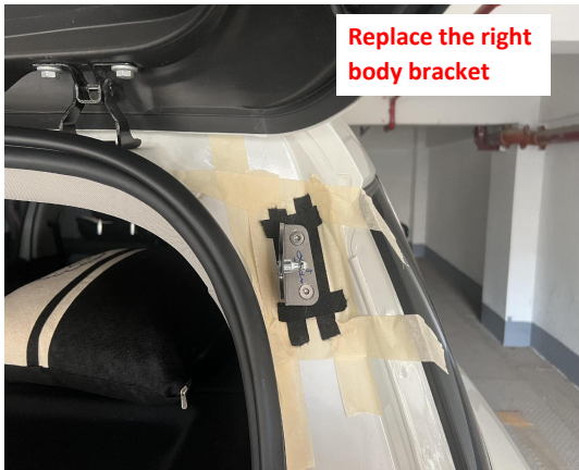
8. Replace the right body bracket.
