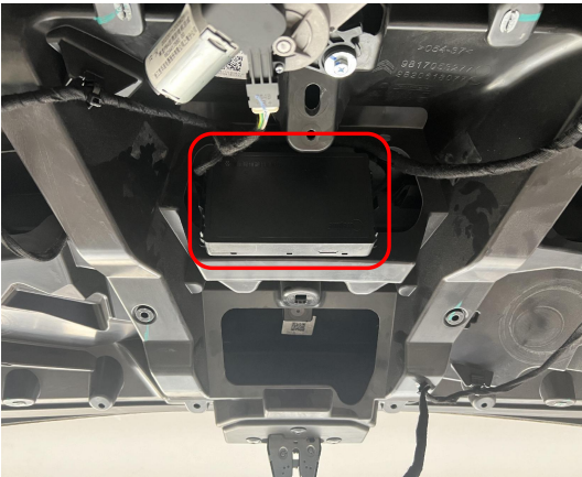
29. Fit the ECU into its bracket and tie the wiring harnesses to the original wiring harness.
