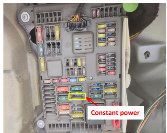
13. The fuse slot for power supply is indicated above.
