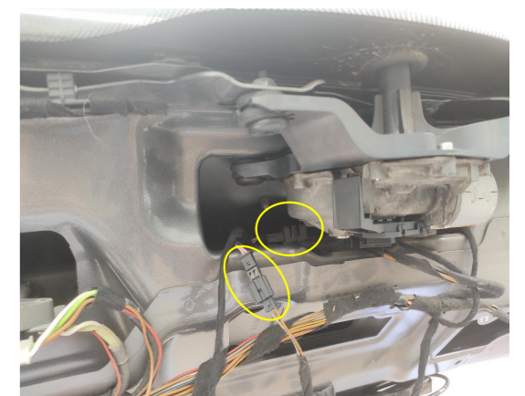
11. Connect the plugs of the lock signal harness to the plugs of the original tailgate switch and the added switch.
