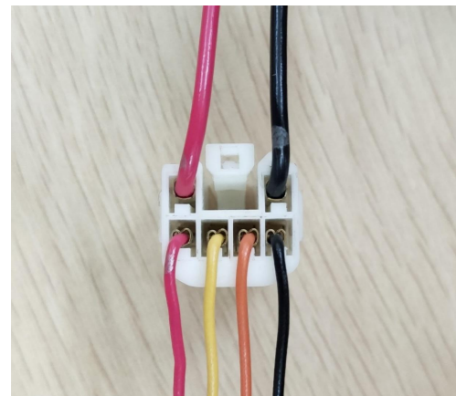
7. Insert the strut wiring harness terminals into the wiring harness connector.
