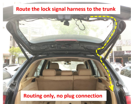
8. Route the lock signal harness to the trunk.
