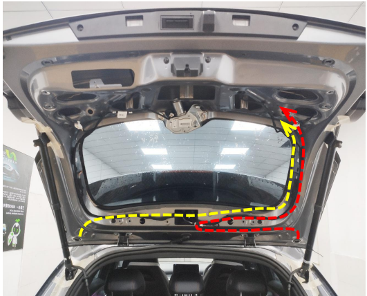
7. Route the left and right strut wiring harnesses to the tailgate.
