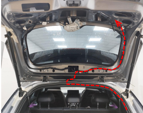
14. Thread the power harness to the tailgate. (no power connection before inserting terminals into the wiring harness connector)
