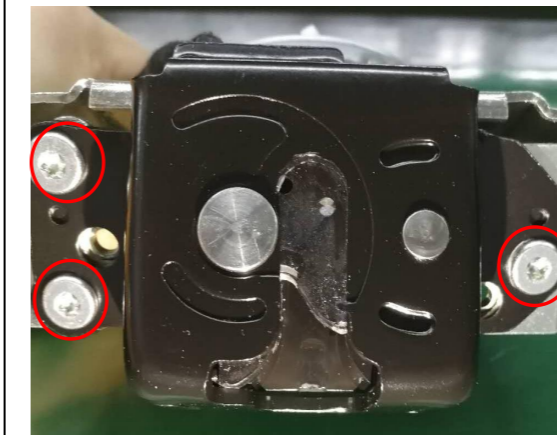
5. Remove the indicated screws from the latch.
