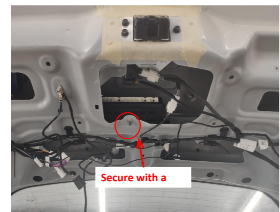
23. Secure the ECU bracket at the indicated position with a nut.
