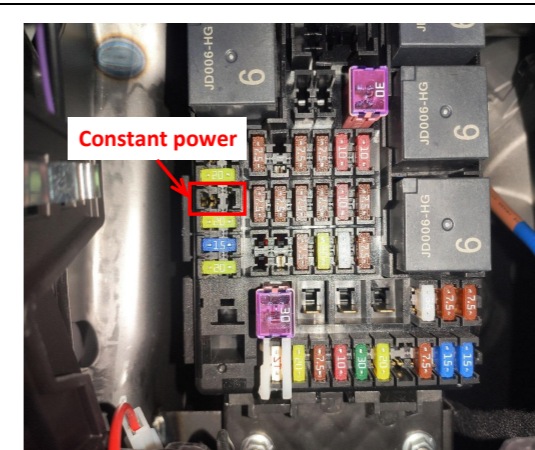
20. The fuse slot for power supply is indicated.
