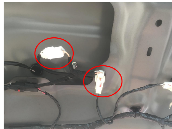
7. Connect the plugs of the lock signal harness to the plugs of original tailgate switch.
