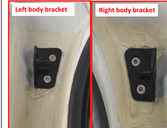
10. Replace the body brackets.
