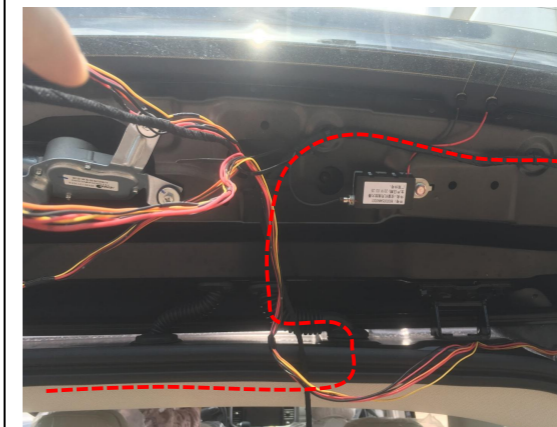
15. Thread the power harness into the tailgate (no plug connection before inserting terminals into the connector).
