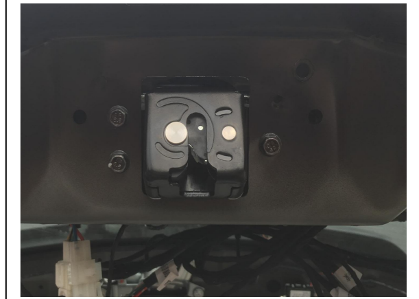
6. Remove the original latch and install our power latch.
