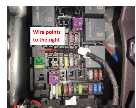
21. Plug the fuse tap into the fuse box and pay attention to the direction of wire.
