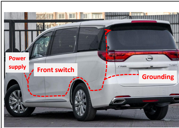
17. Route the power harness as indicated.
