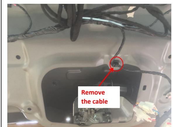
22. Remove the indicated cable clip for installing the ECU bracket.
