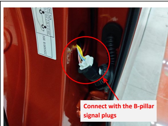
18. Connect the plugs of the power harness with the B-pillar signal plugs.
