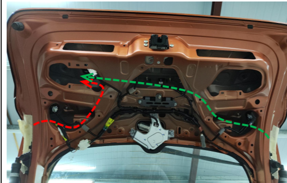
9. Route the strut wiring harnesses.
