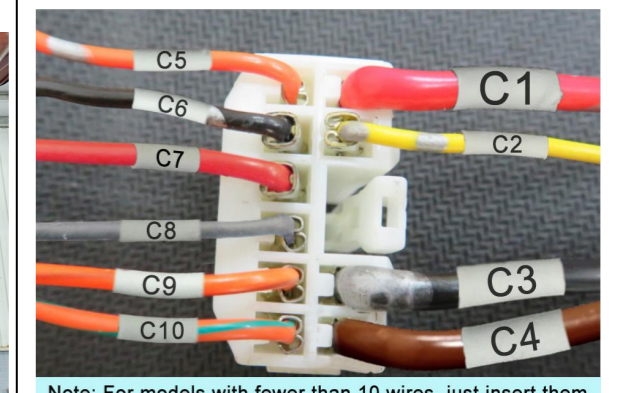
16. Insert the power harness terminals into the wiring harness connector.
