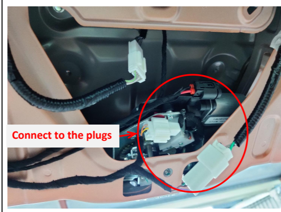
13. Connect the plugs of the lock signal harness to the plugs of the lock actuator.
