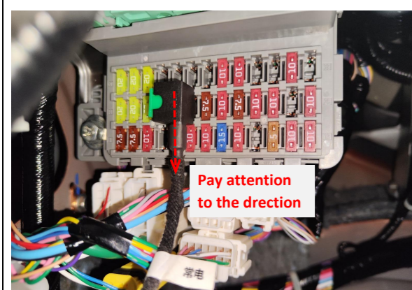
22. Plug the fuse tap into the fuse box and pay attention to the direction.
