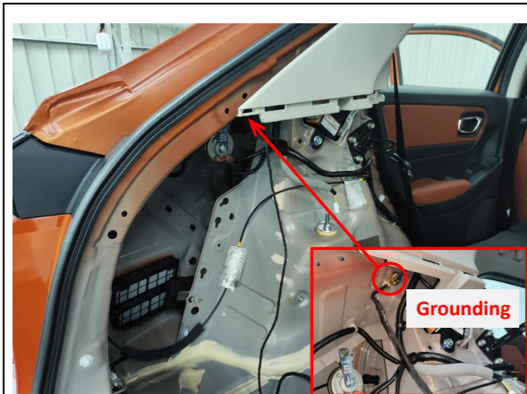
17. Ground at the left side of the trunk.
