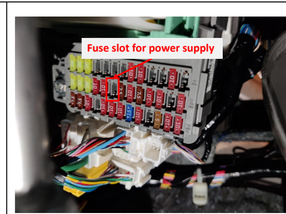
21. The fuse box is located beside the pedals and the fuse slot for power supply is indicated above.
