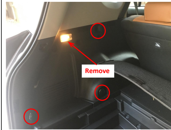
5. Remove the trim panel on the left side of the trunk.
