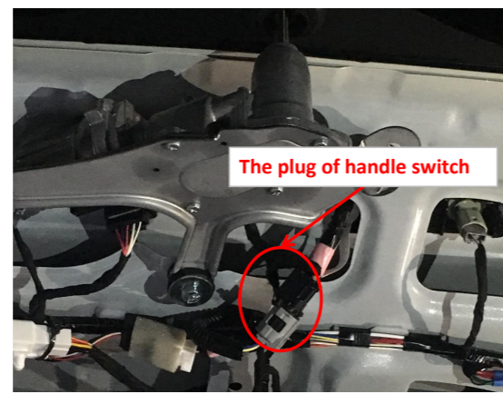
8. Connect the lock signal harness to the plugs of tailgate handle switch.
