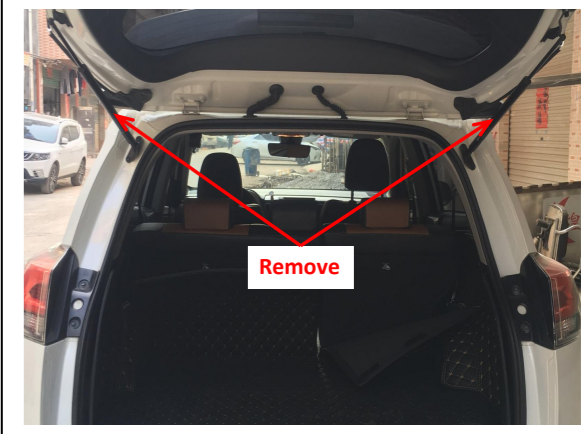
11. Remove the original gas struts.
