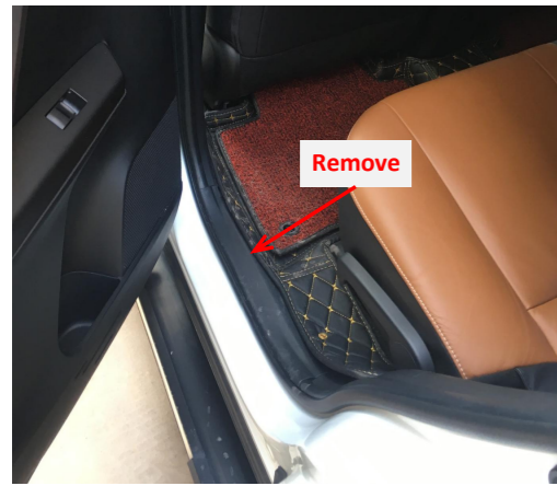
2. Remove the rear left side door sill panel.
