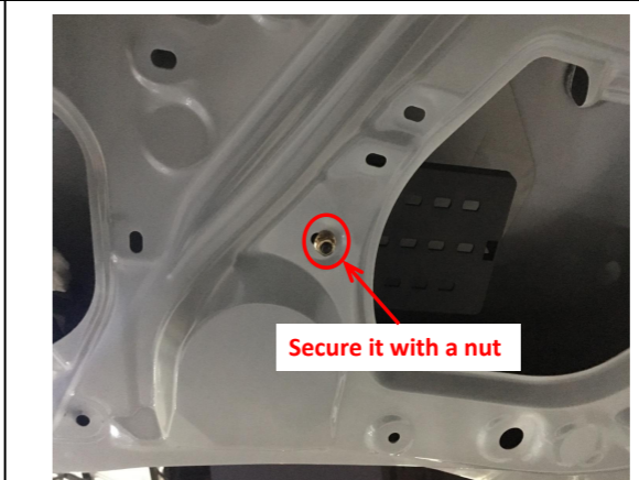
25. Secure the ECU bracket at the indicated hole on the left side of tailgate.
