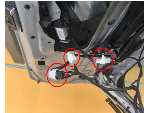
9. Connect the lock signal harness to the plugs of the power latch.
