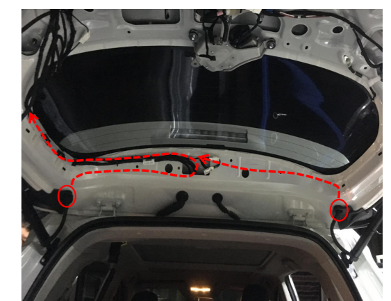
16. Route the strut wiring harnesses.
