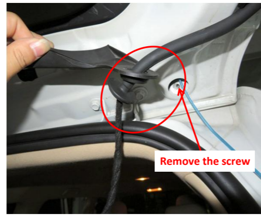
19. Remove the screw from the hole and thread the strut wiring harness through the hole.
