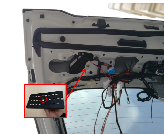
30. Screw a nut on the ECU bracket first and then fix it to the indicated hole.
