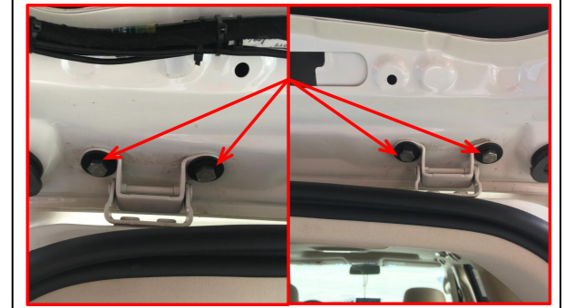
1. Add the reinforcing washers to the hinges and secure them with provided screws.
