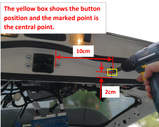
32. Stick the hole template to the indicated position of tailgate and open a hole for installing the added switch.
