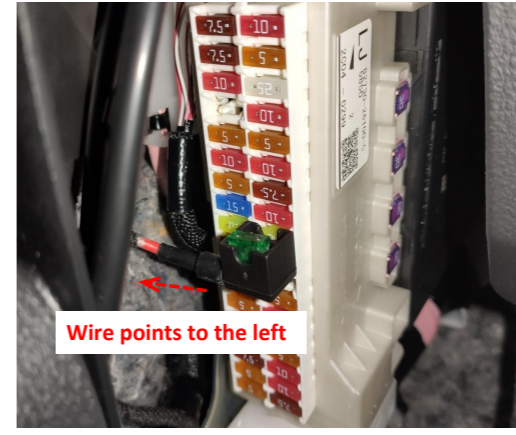
25. Plug the fuse tap into the fuse box, and pay attention to the direction of wire.
