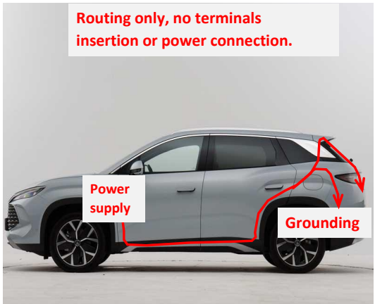
16. Route the power harness to the tailgate.
