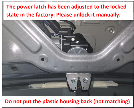
14. Install our power latch and do not put the plastic housing back (not matching).
