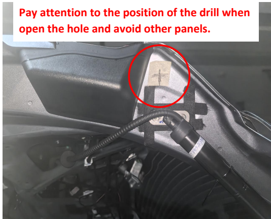
10. Drill a hole at the indicated position on both side with a Ø21mm drill bit to allow strut wiring harness to pass
