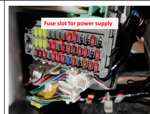
21. The fuse box is located beside the pedals and the fuse slot for power supply is indicated above.
