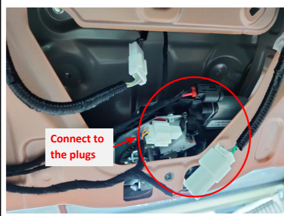
13. Connect the plugs of the lock signal harness to the plugs of the power latch
