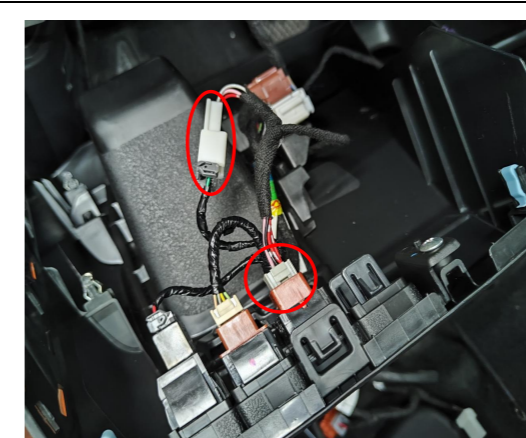
20. Connect the plugs as shown above.
