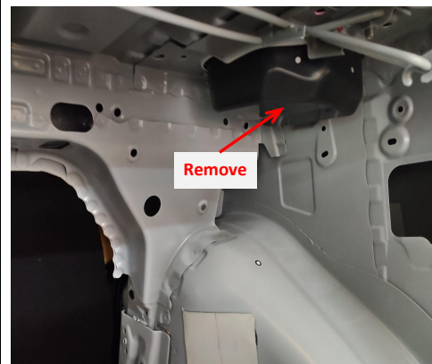
5. Remove the plastic boxes of seat belt on both sides (remember to install them back after finishing the installation).
