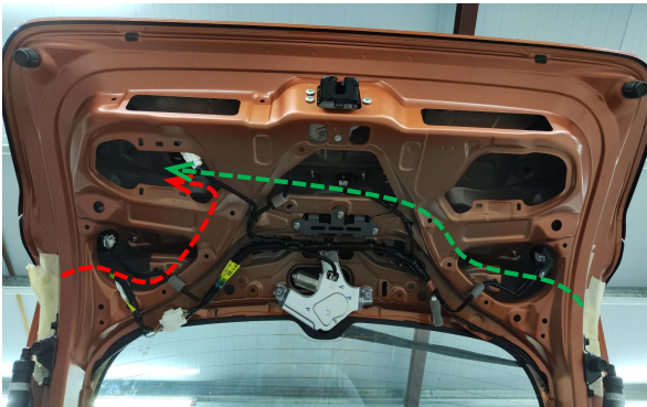
9. Route the strut wiring harnesses.
