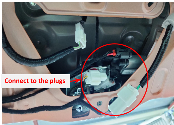
13. Connect the plugs of the lock signal harness to the plugs of the lock actuator.
