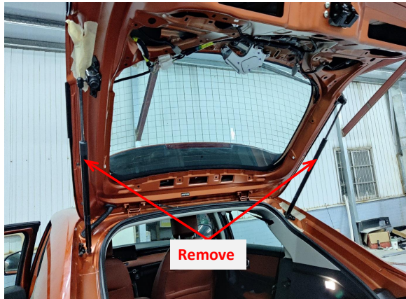
5. Remove the original gas struts.
