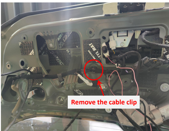
22. Remove the indicated cable clip.
