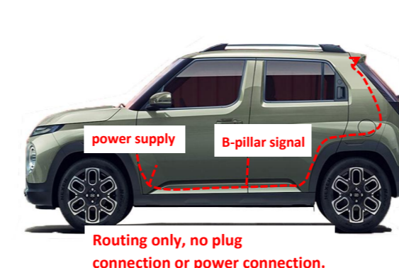
14. Route the power harness as indicated (if you need to install the added front switch, route the switch wiring harness in the same way).
