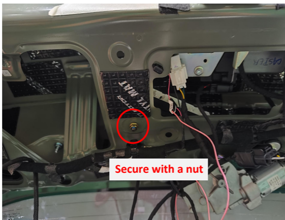
23. Secure the ECU at the hole with a nut.
