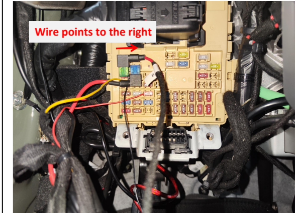
21. Plug the fuse tap into the fuse box and pay attention to the direction.
