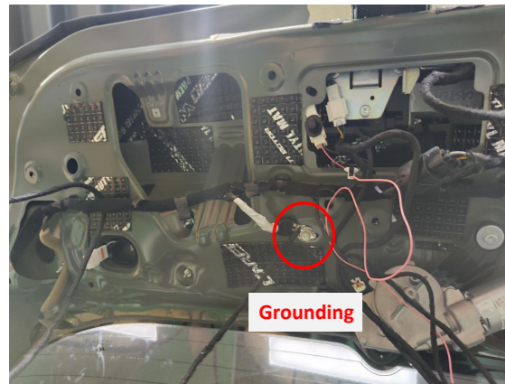
17. Ground at the indicated position.
