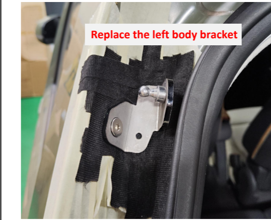
5. Replace the left body bracket.
