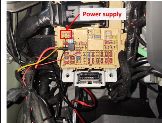
20. The fuse box is located at the driver's area and the fuse slot for power supply is indicated above.
