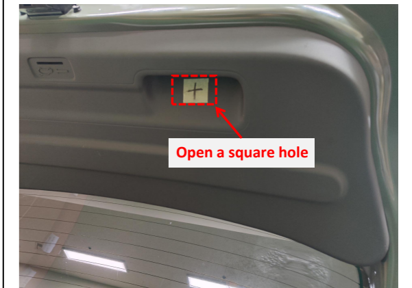
26. Open a square hole at the indicated position of the tailgate trim panel for the added tailgate switch.
