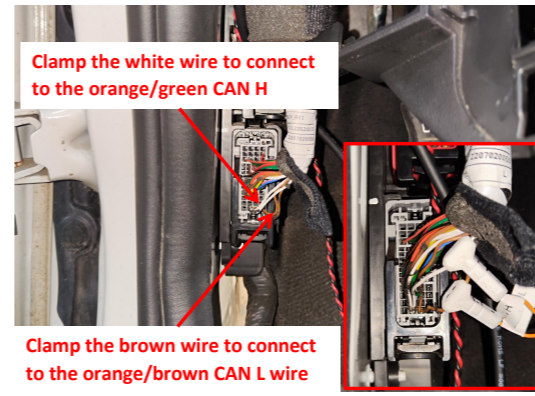
19. Connect the CAN signal: Clamp the white wire to connect to the orange/green CAN H and brown wire to the orange/brown CAN L wire
