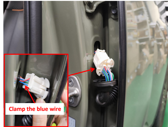
18. Connect the B-pillar signal: clamp the indicated blue wire to connect to the orange wire of the power harness.
